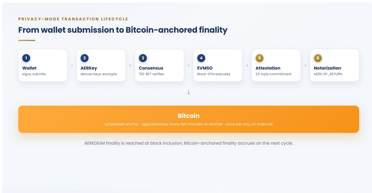
Figure 3. Privacy-mode transaction lifecycle, from wallet submission to Bitcoin-anchored finality
