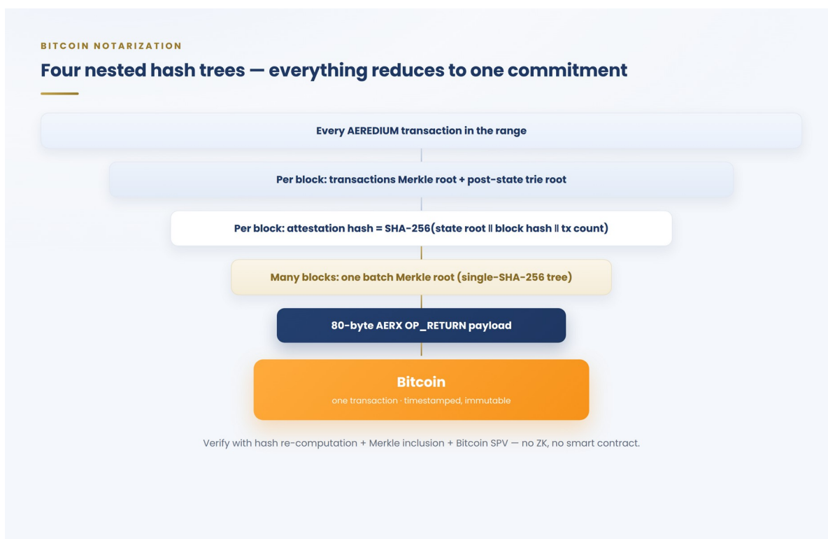
Figure 8. Bitcoin notarization — four nested hash trees reduce to one commitment
