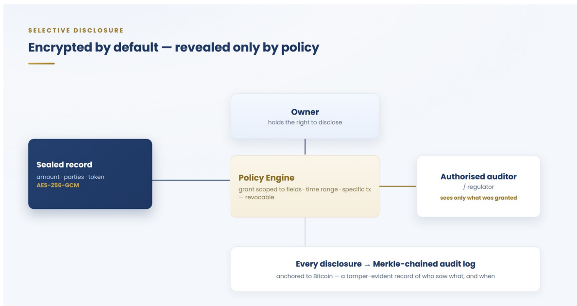
Figure 5. Selective disclosure — encrypted by default, revealed only by policy
