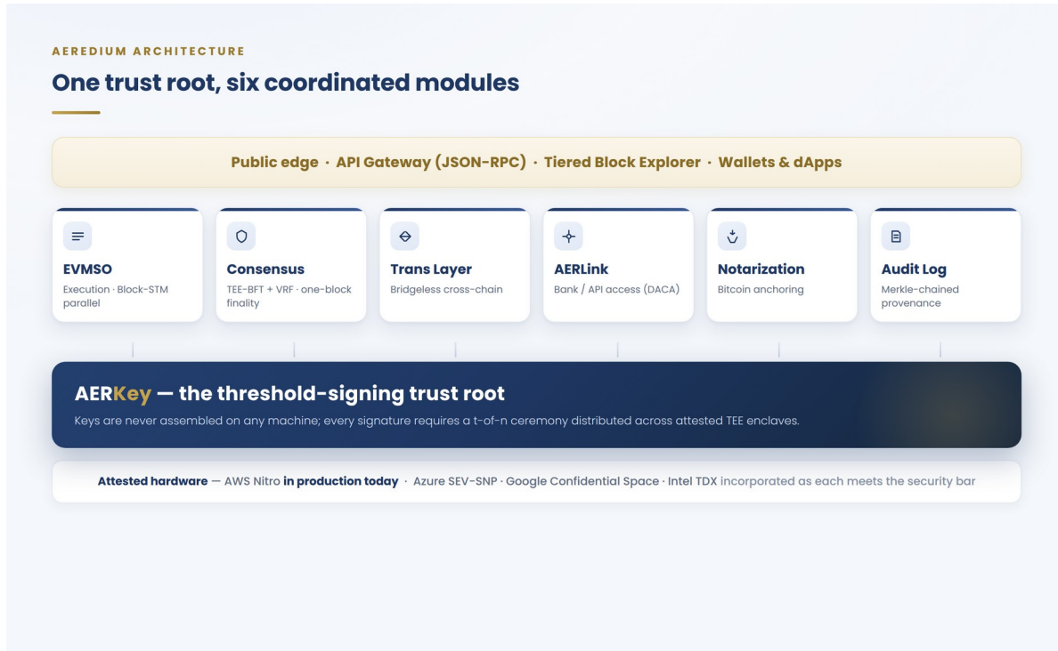
Figure 2. AEREDIUM architecture — one trust root, six coordinated modules
